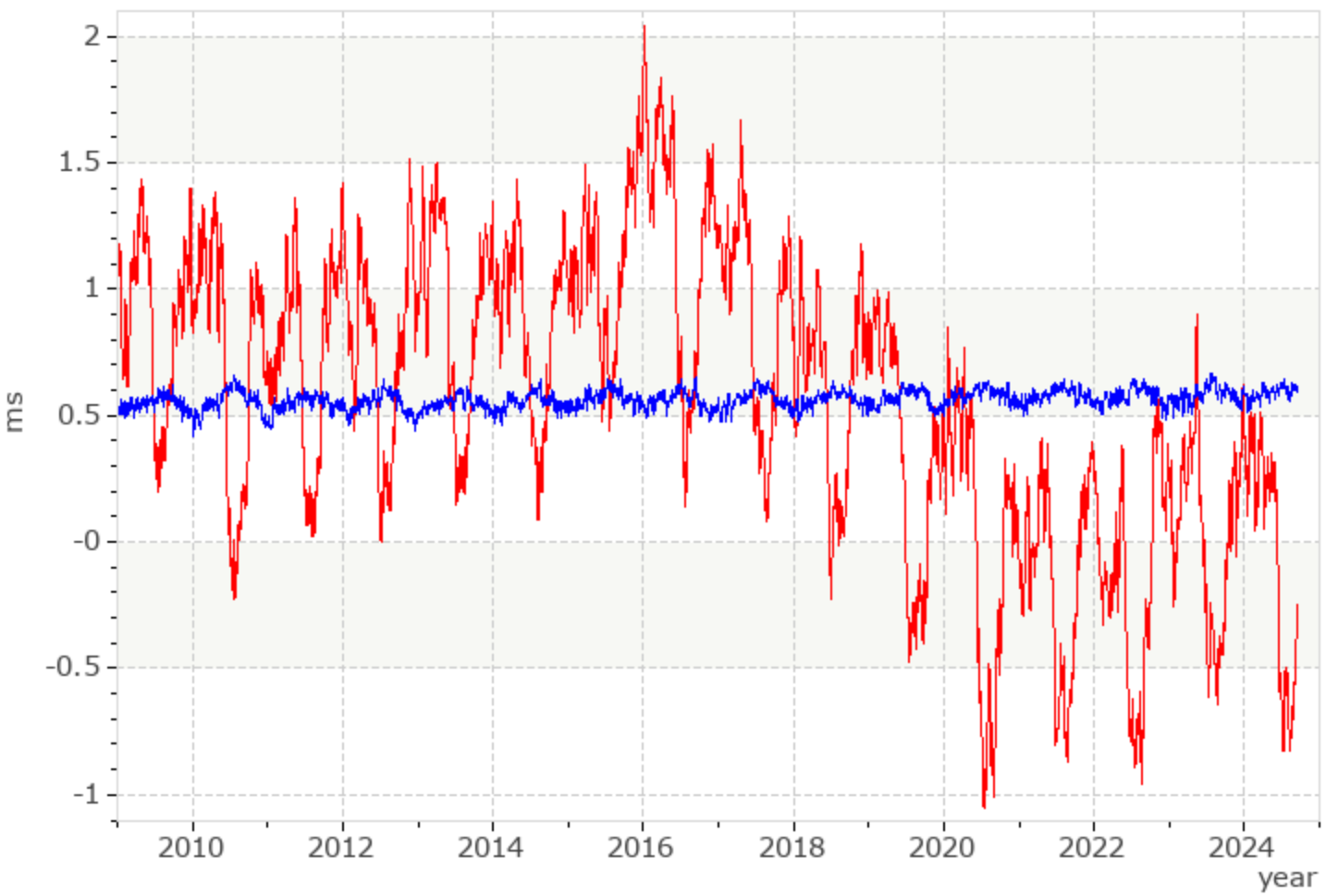
Length of day change
