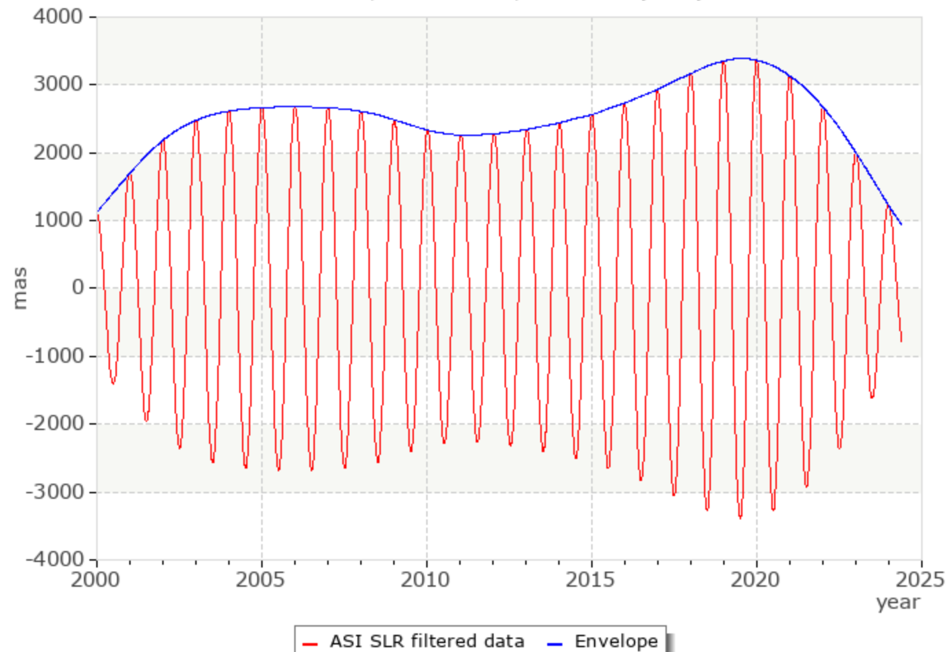
Panteleev band pass filter of deps around 1 cycle / year
