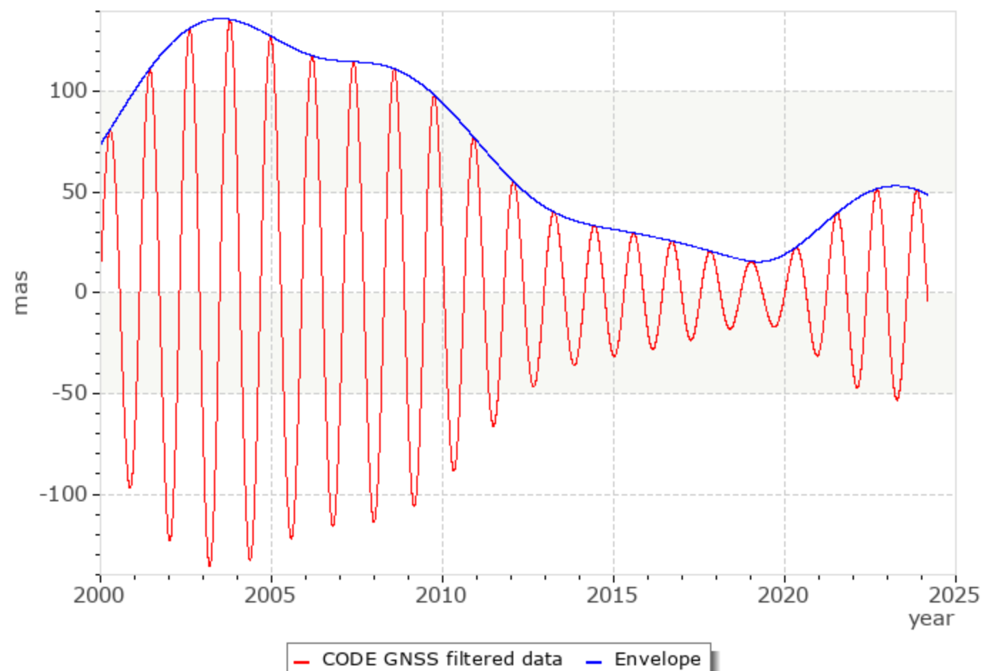
Panteleev band pass filter of x - i y around 0.845 / year
