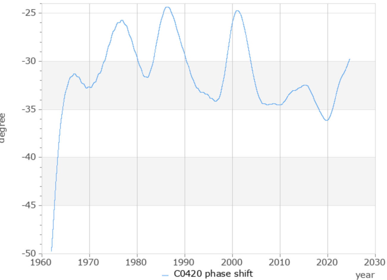
Panteleev band pass filter of LOD / 86400 s SI around 1 cycle / year
