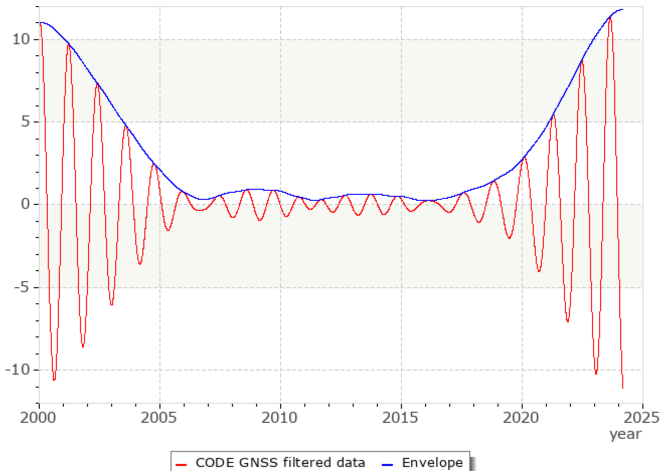
Panteleev band pass filter of x - i y around -0.845 / year
