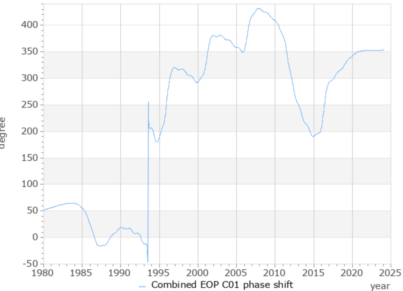
Panteleev band pass filter of x - i y around -0.845 / \text{year}
