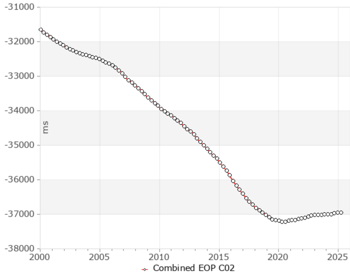
UT1-TAI
