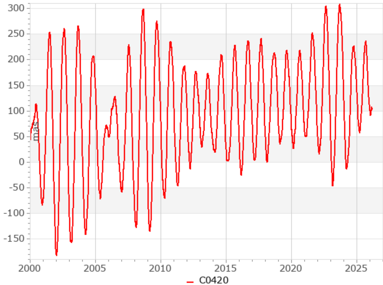
Polar coordinate x IERS Earth Orientation Centre
