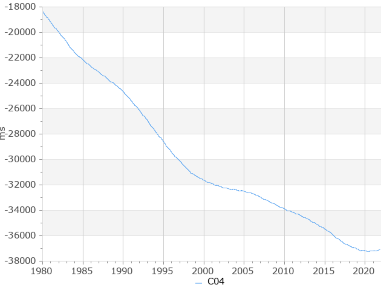
UT1-TAI
