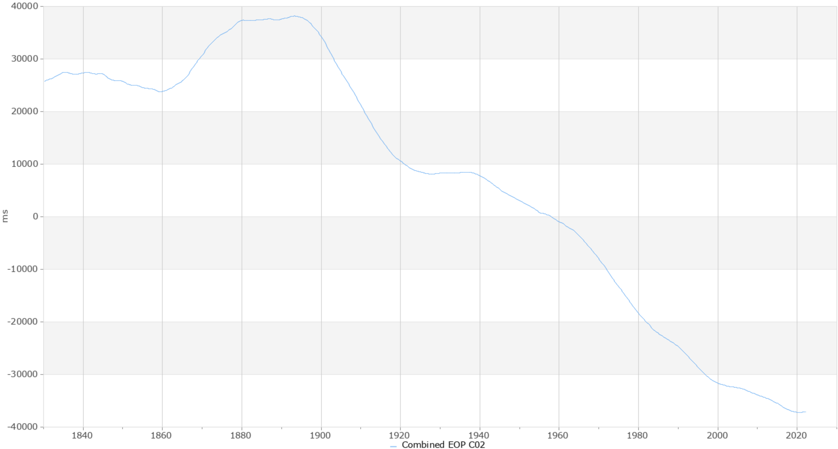
UT1-TAI
