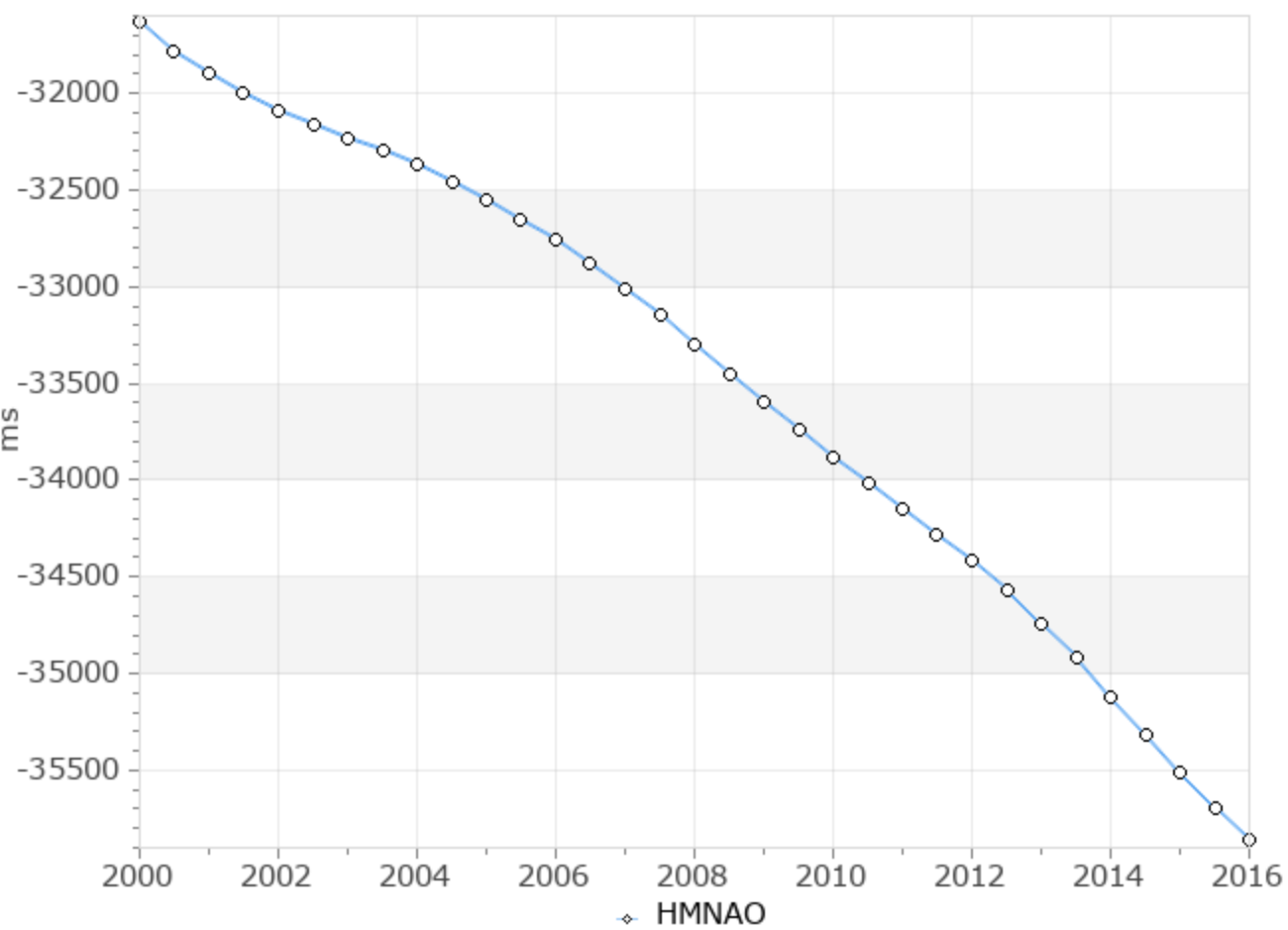
UT1-TAI
