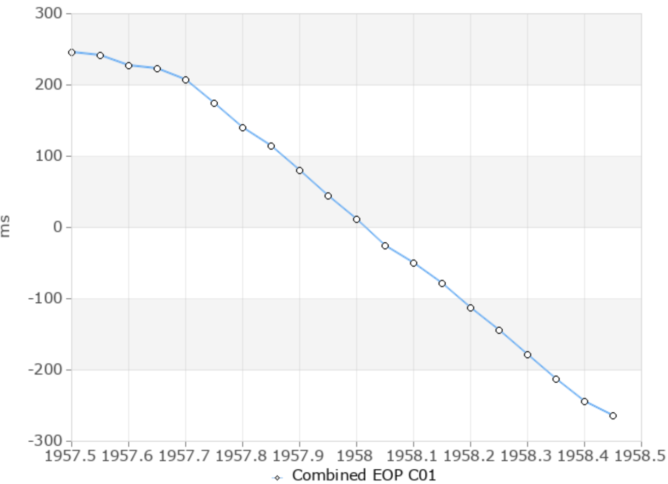
UT1-TAI
