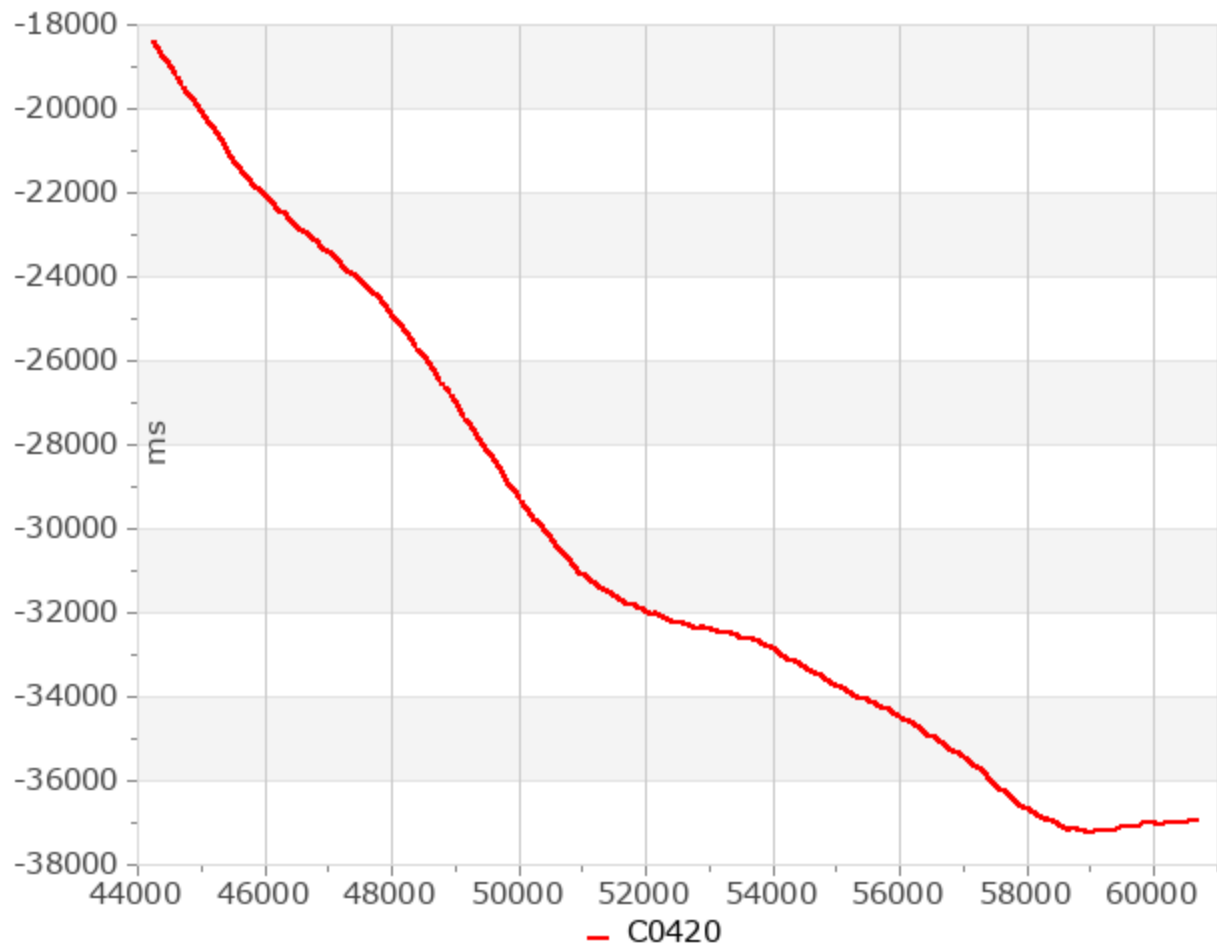
UT1-TAI
