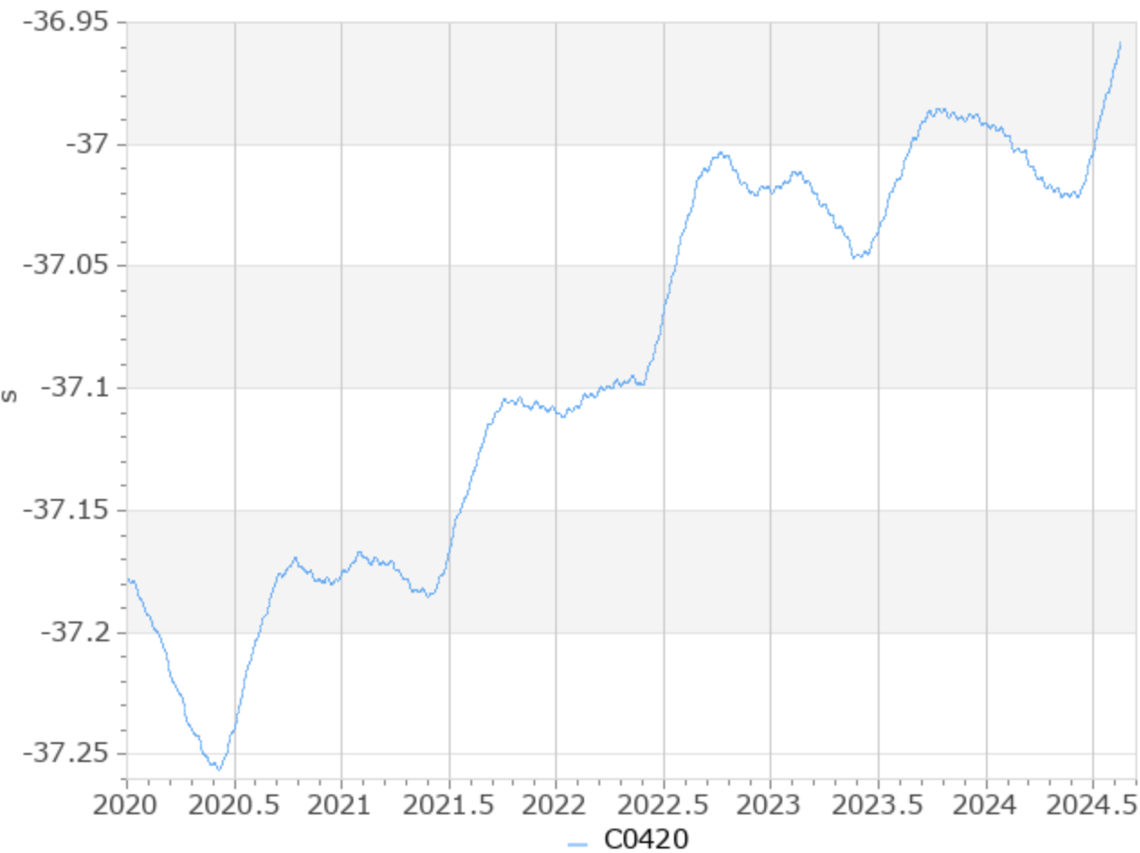
UT1-TAI
