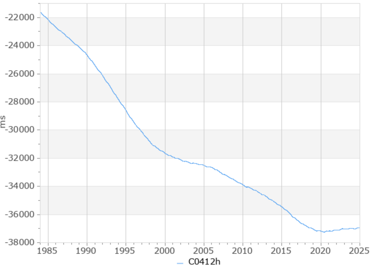
UT1-TAI
