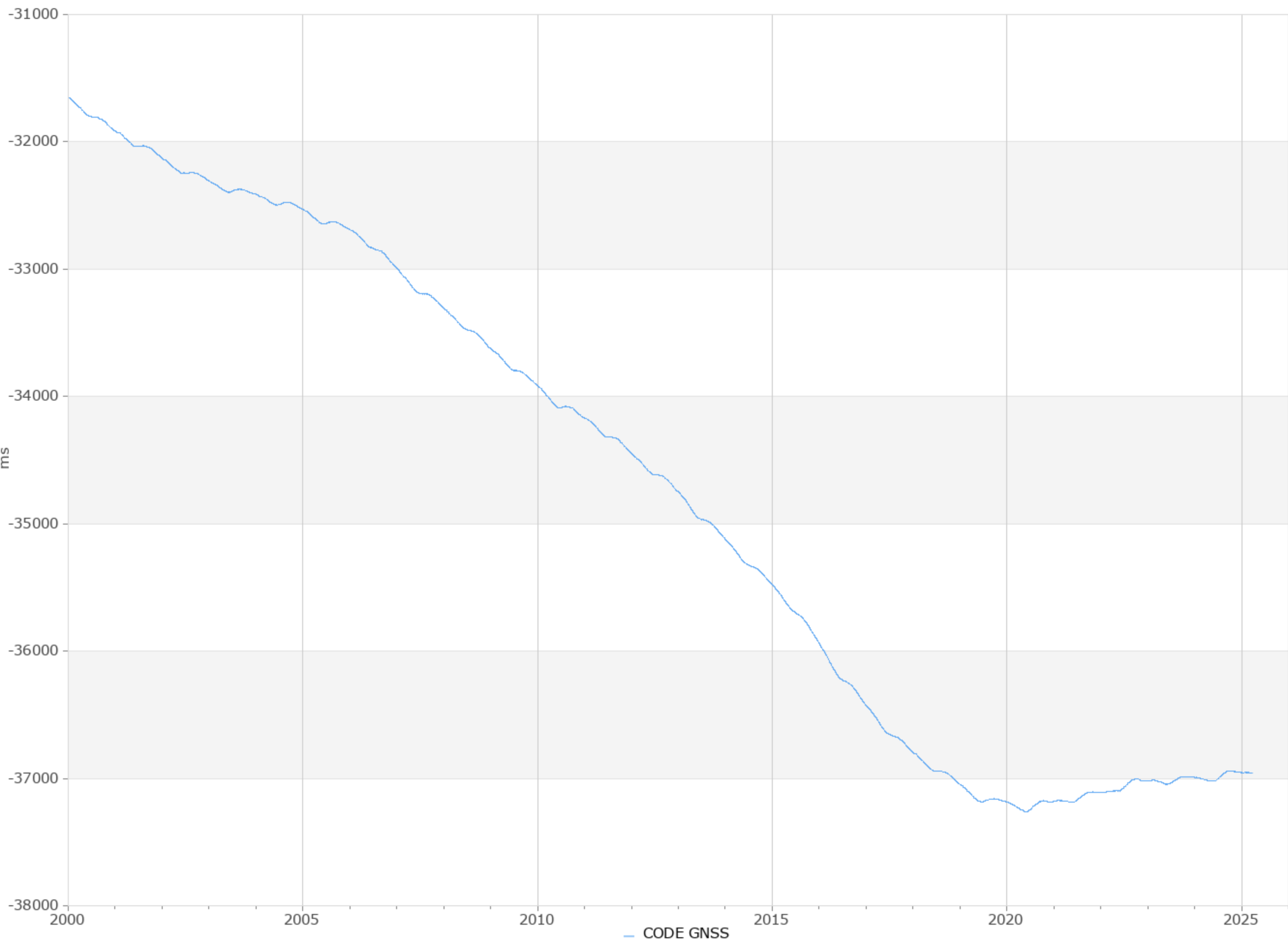
UT1-TAI
