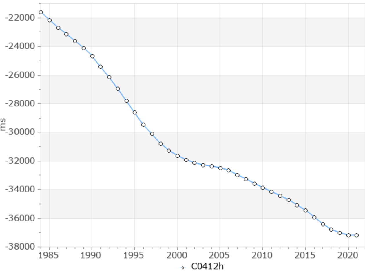
UT1-TAI
