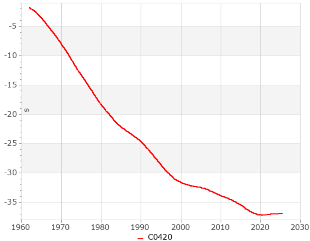
UT1-TAI
