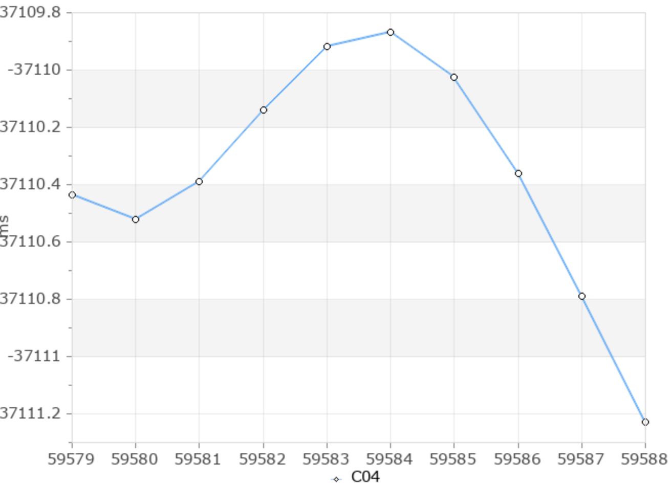
UT1-TAI
