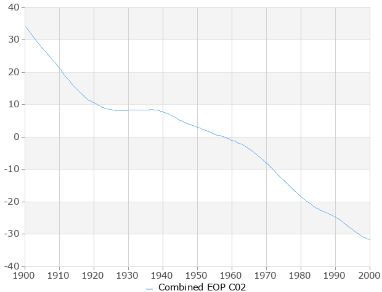
UT1-TAI
