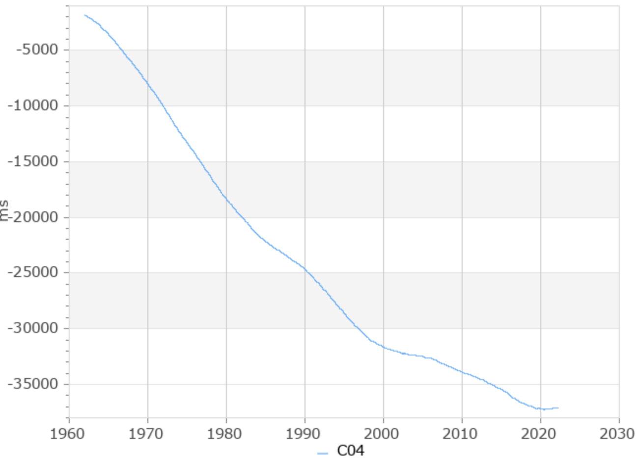
UT1-TAI
