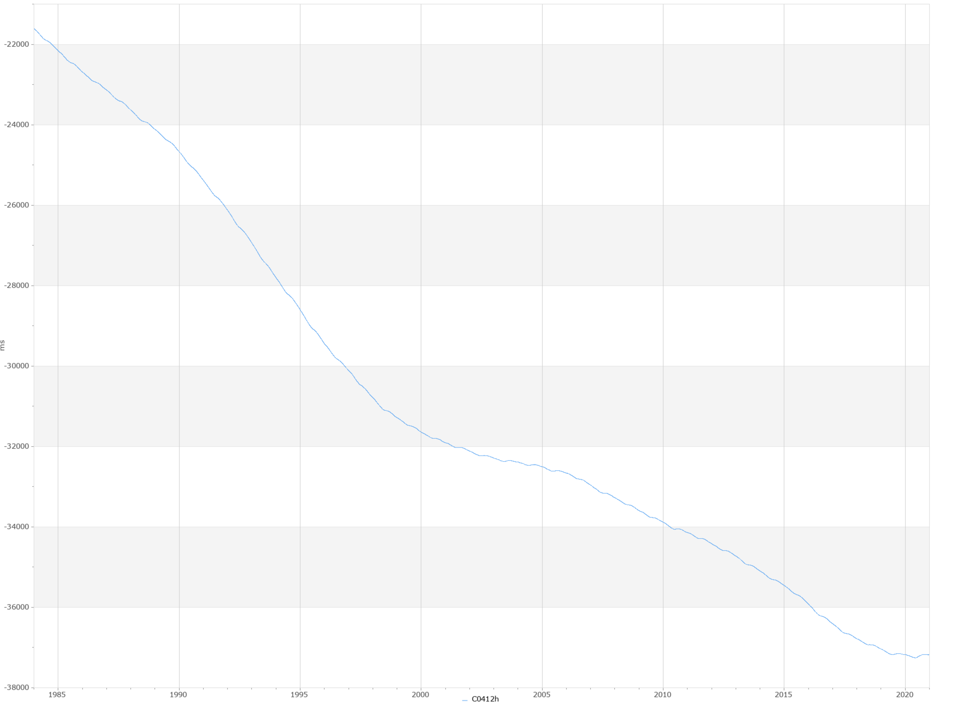
UT1-TAI
