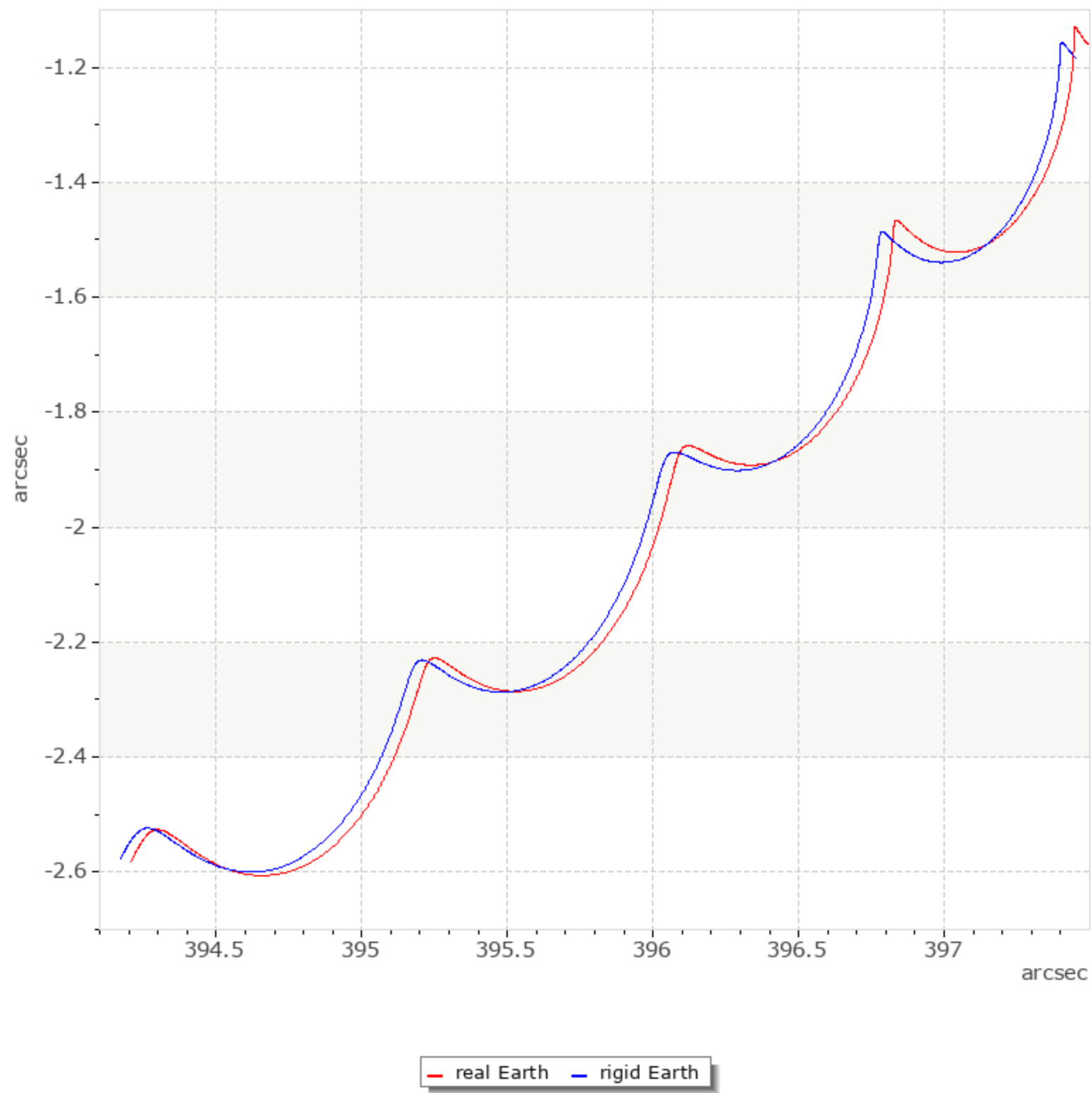
Real Earth and rigid Earth figure axes projected on the equatorial plane of the epoch J2000
