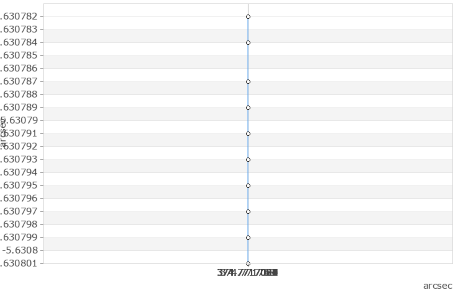
Geographic axis projected on the equatorial plane J2000
