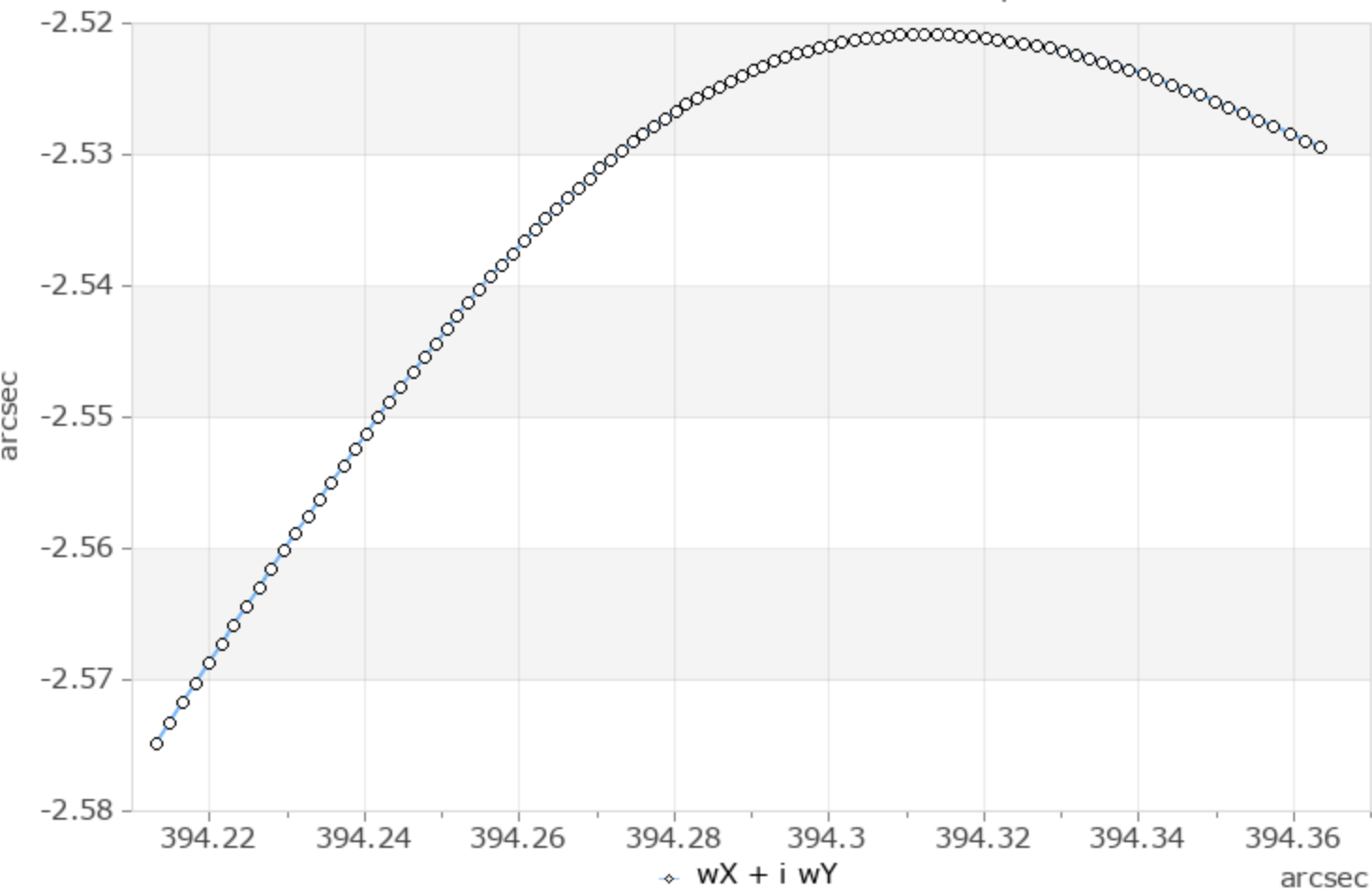
Motion of the instantaneous rotation vector in the XY plane of the ICRF
