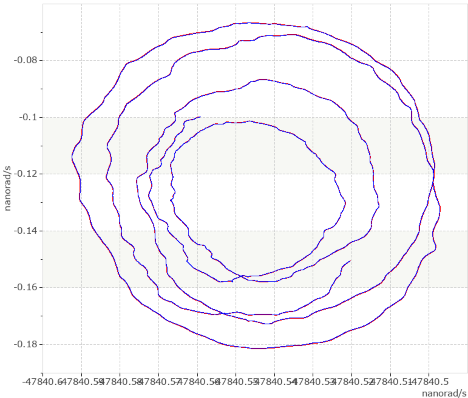
Instantaneous and mean rotation vector components ( w_x , w_y ) in the local xy plane
