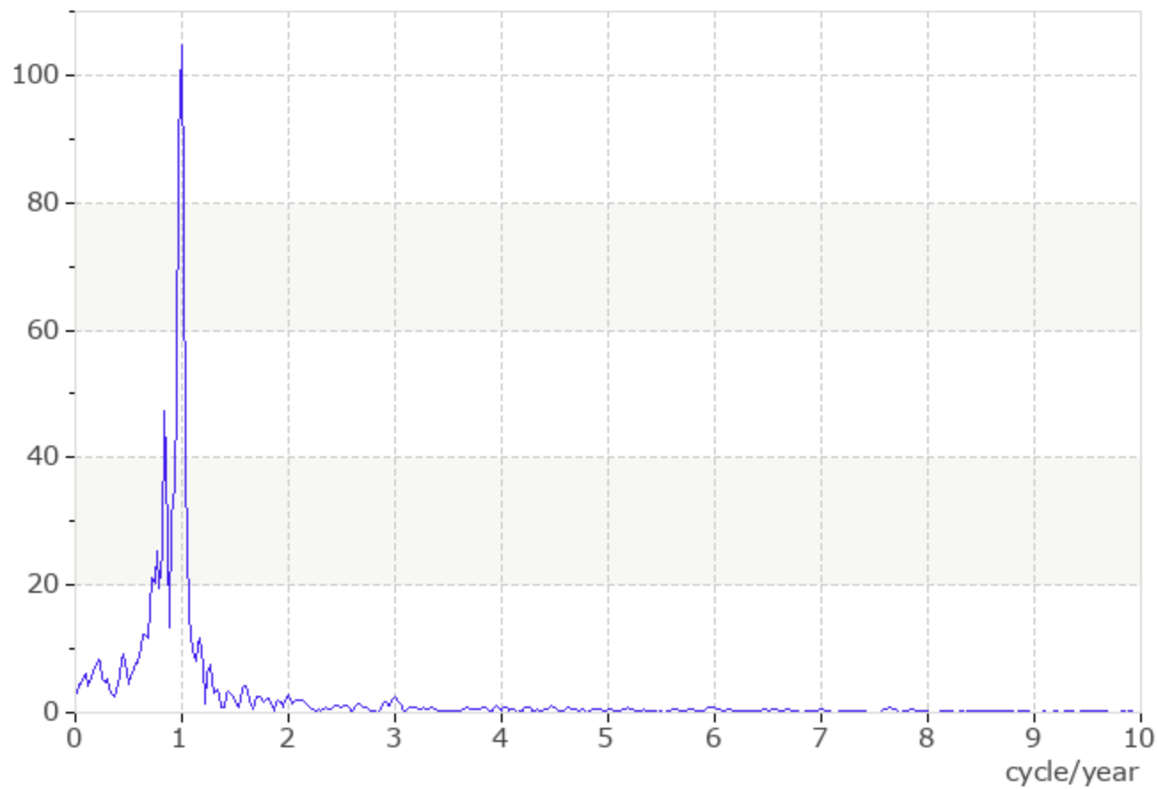
Polar coordinate x
