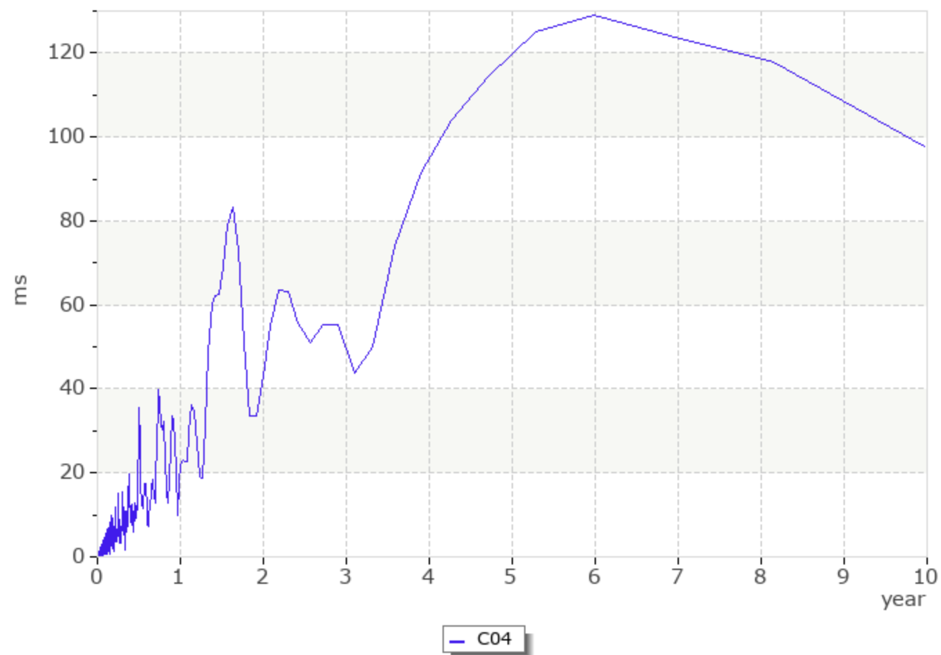
UT1-UTC
