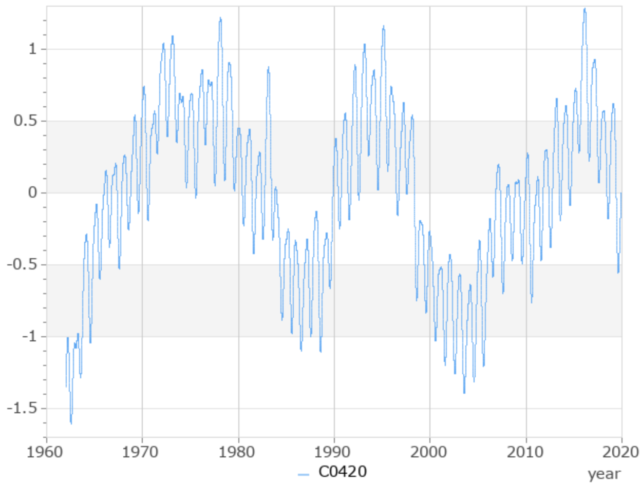
Vondrak filter of LOD / 86400 s SI
