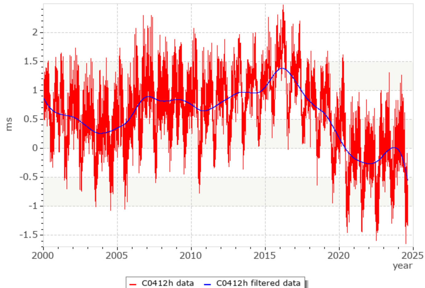
Vondrak filter of LOD / 86400 s SI
