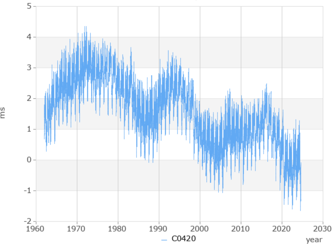
Vondrak filter of LOD / 86400 s SI
