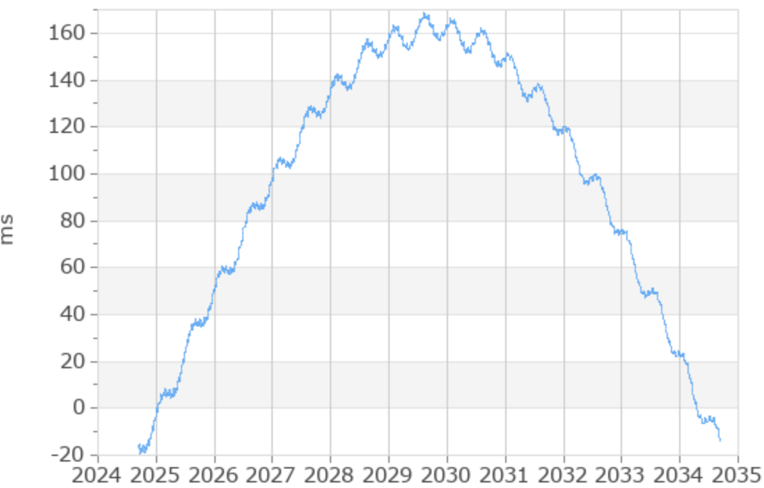
Effect of the zonal tide on UT1
